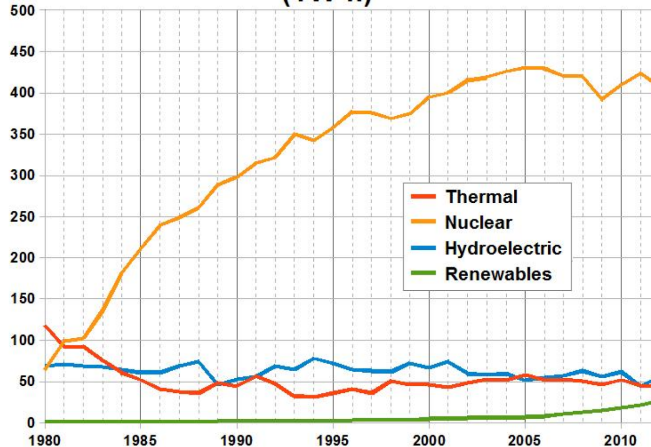
Electricity Production in France by Source (TW-h)
