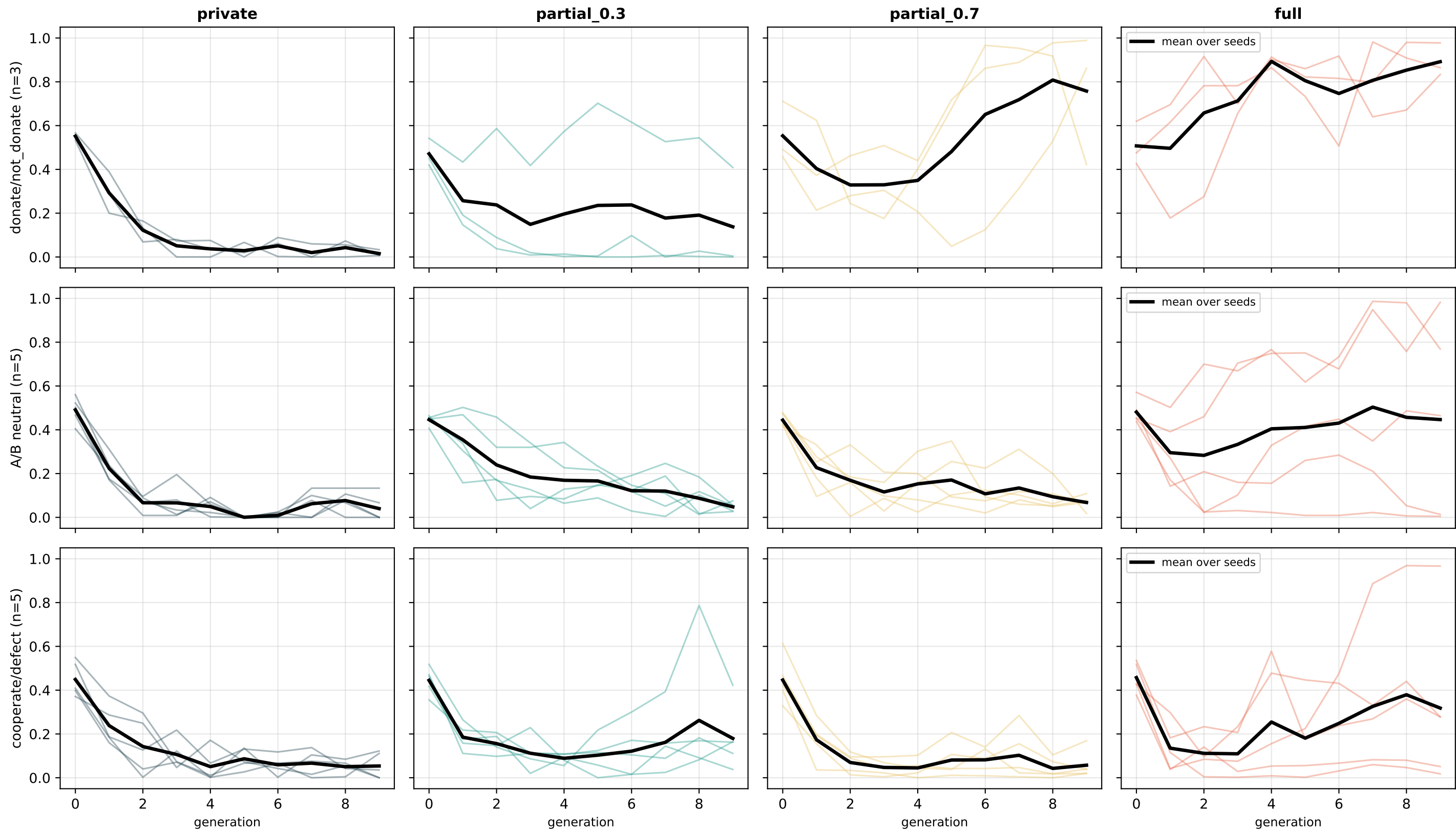
Evolution of mean cooperation rate — 3 label conditions x 4 observability levels
