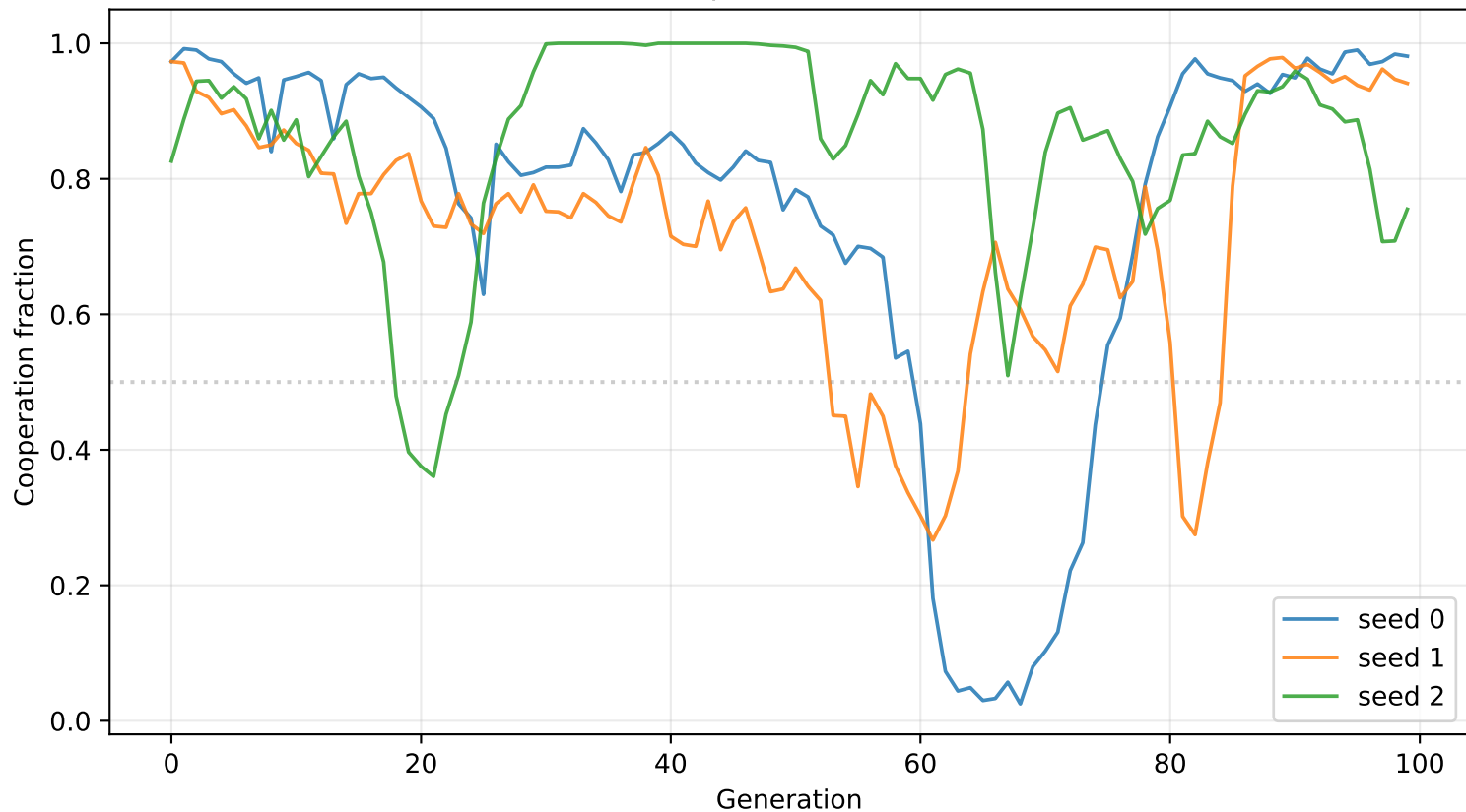
Fermi Z-like (LLM \mu +small-mutate), 3 seeds \times 100 gen \times 1000 inter final coop = 0.892 \pm 0.098
