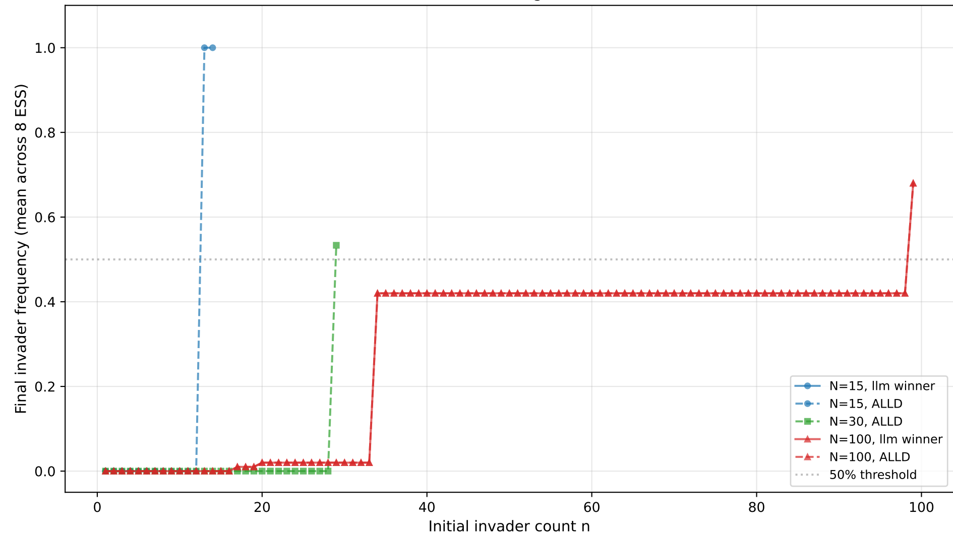
Invasion threshold WITH burn-in=10 (all-good initial state): n^* scales with N
