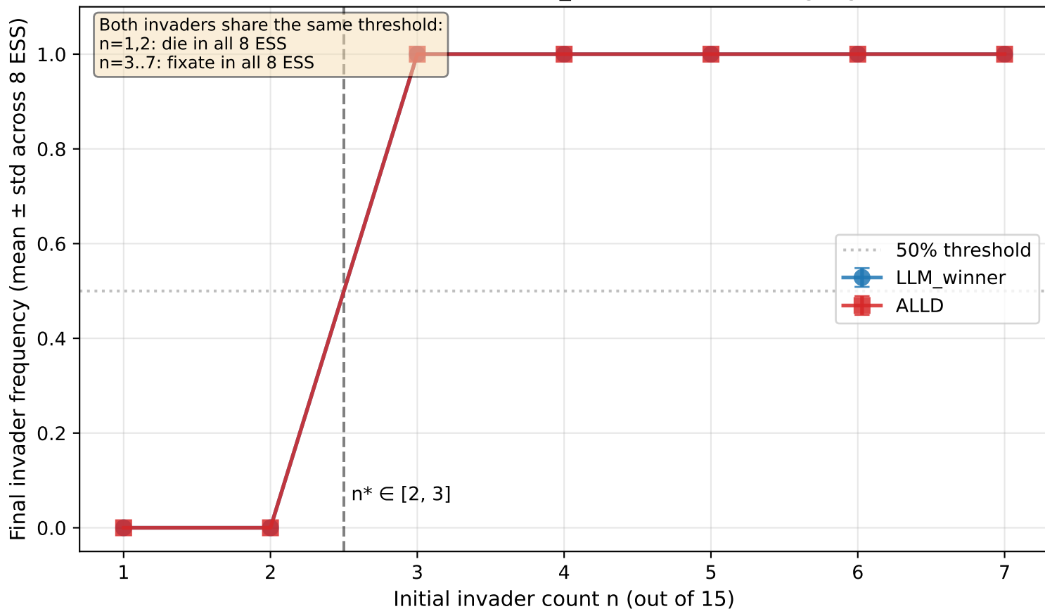
Invasion threshold: ALLD vs LLM_winner across leading-eight ESS
