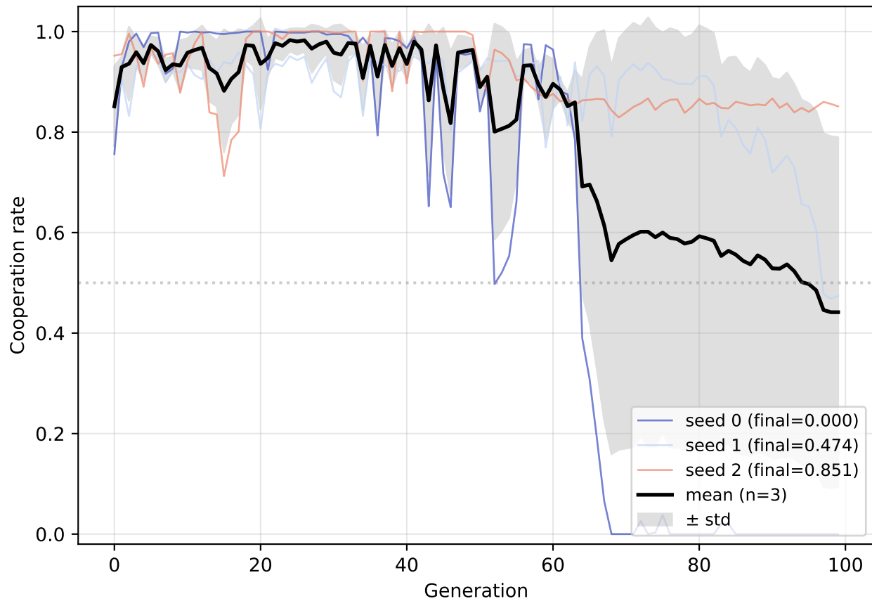
100 gen × 1000 inter × 3 seeds (type-2 LLM)
