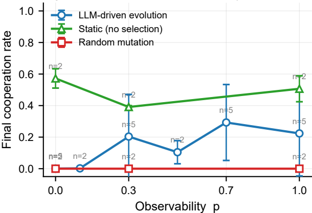
Fig. 2. Cooperation vs observability
