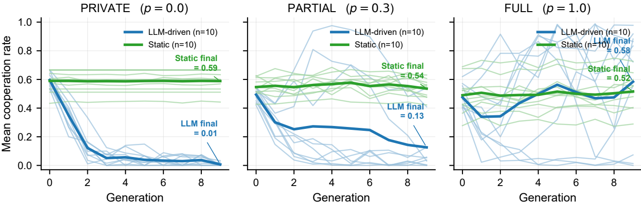
Fig. 4. Selection pressure: LLM-driven evolution vs static control
