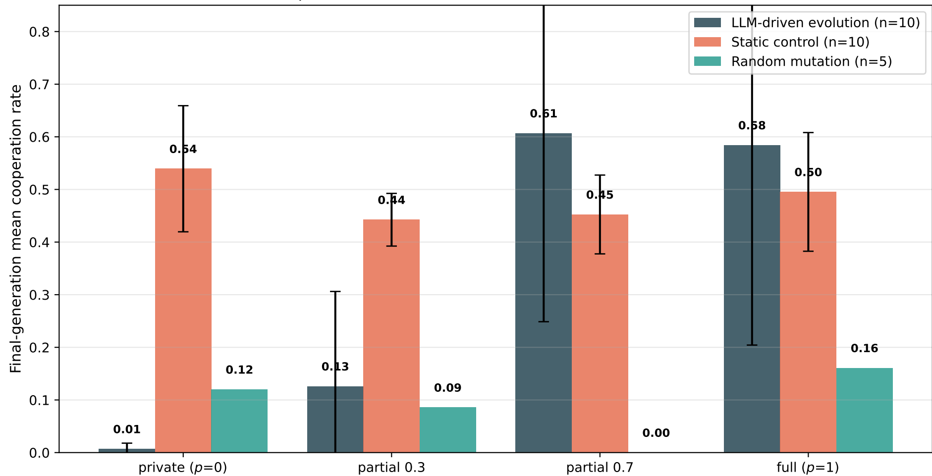
Control comparison (v22 data): LLM-driven vs. static vs. random mutation
