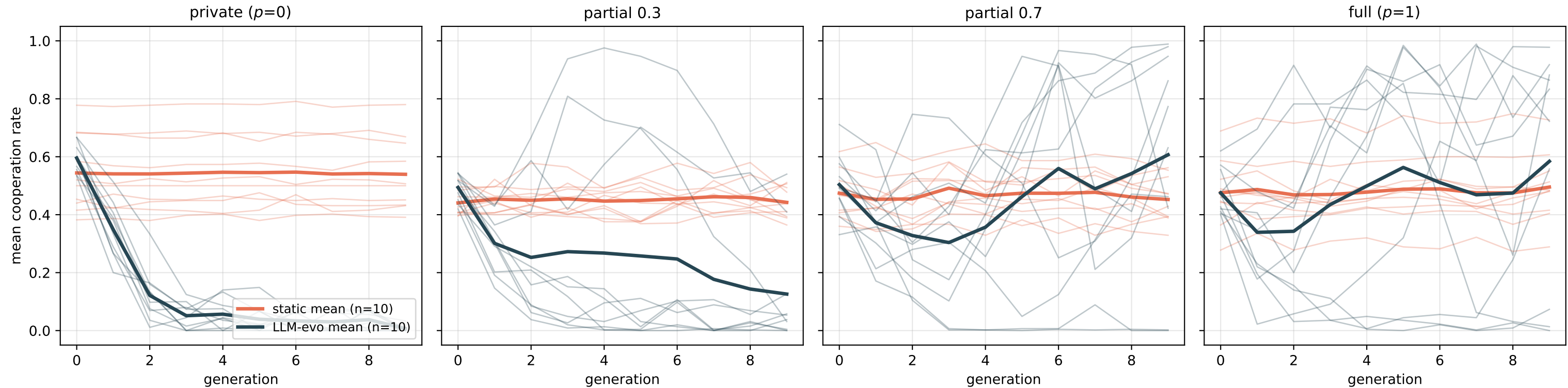
Trajectory comparison (v22 data): LLM-driven evolution vs. static control
