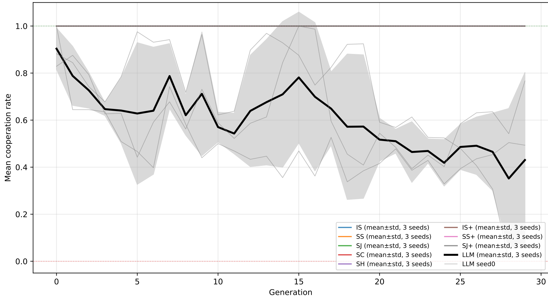
v2 quantitative baseline: 8 leading-eight (Ohtsuki-Iwasa 2006) vs LLM-evolved (full observability, n=15, 30 rounds/gen, 30 generations)
