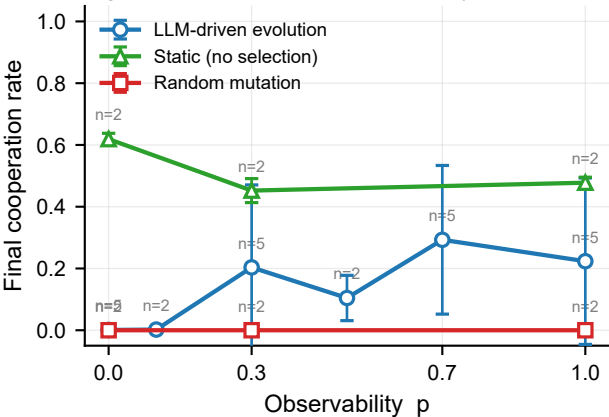
Fig. 2. Cooperation vs observability
