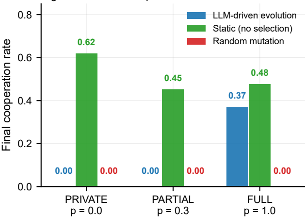
Fig. 3. Control comparison
