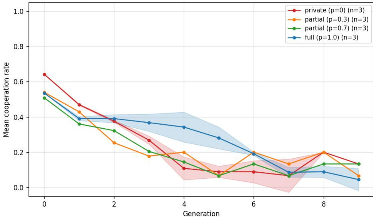
Cooperation trajectories across observability conditions (Exp 1, G=10 , N=15 )
