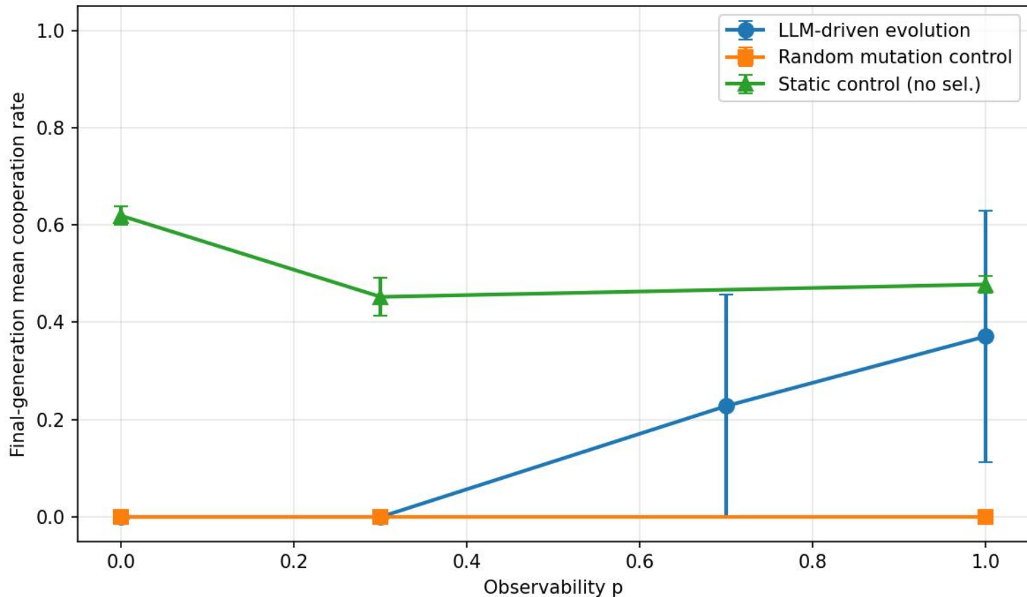
Fig 2: Cooperation vs Observability (LLM-evo vs controls)
