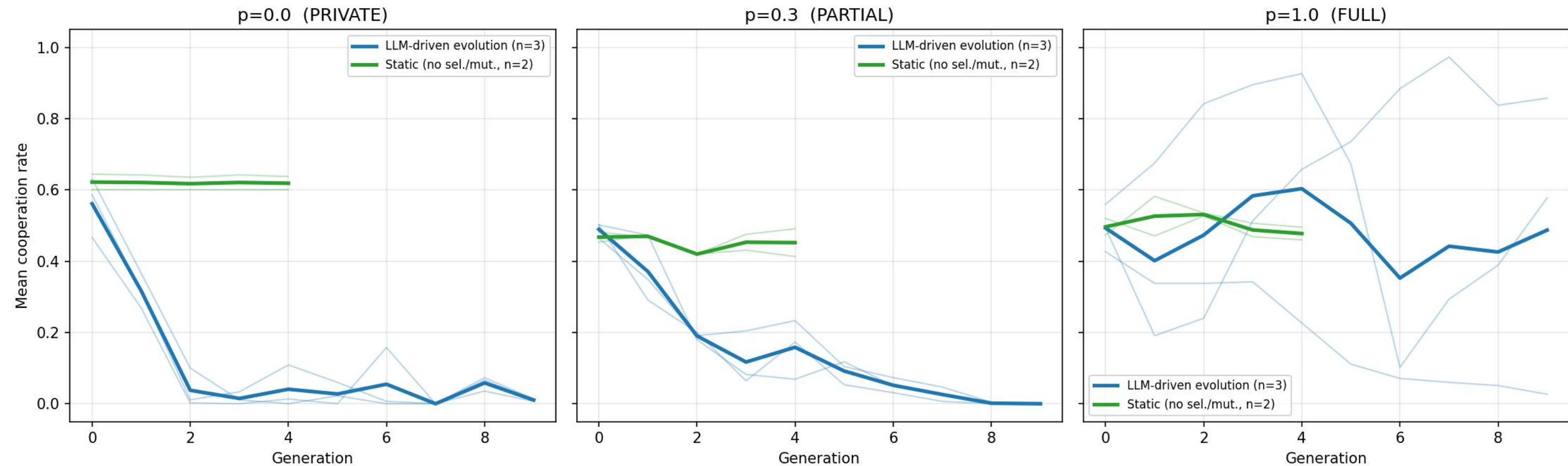
Fig 4: Selection Pressure — LLM-driven Evolution vs Static Control
