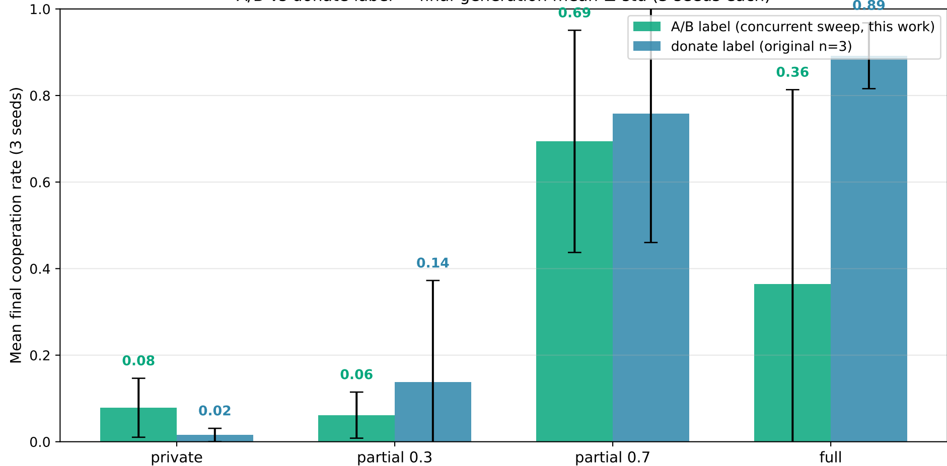
A/B vs donate label — final-generation mean \pm std (3 seeds each)
