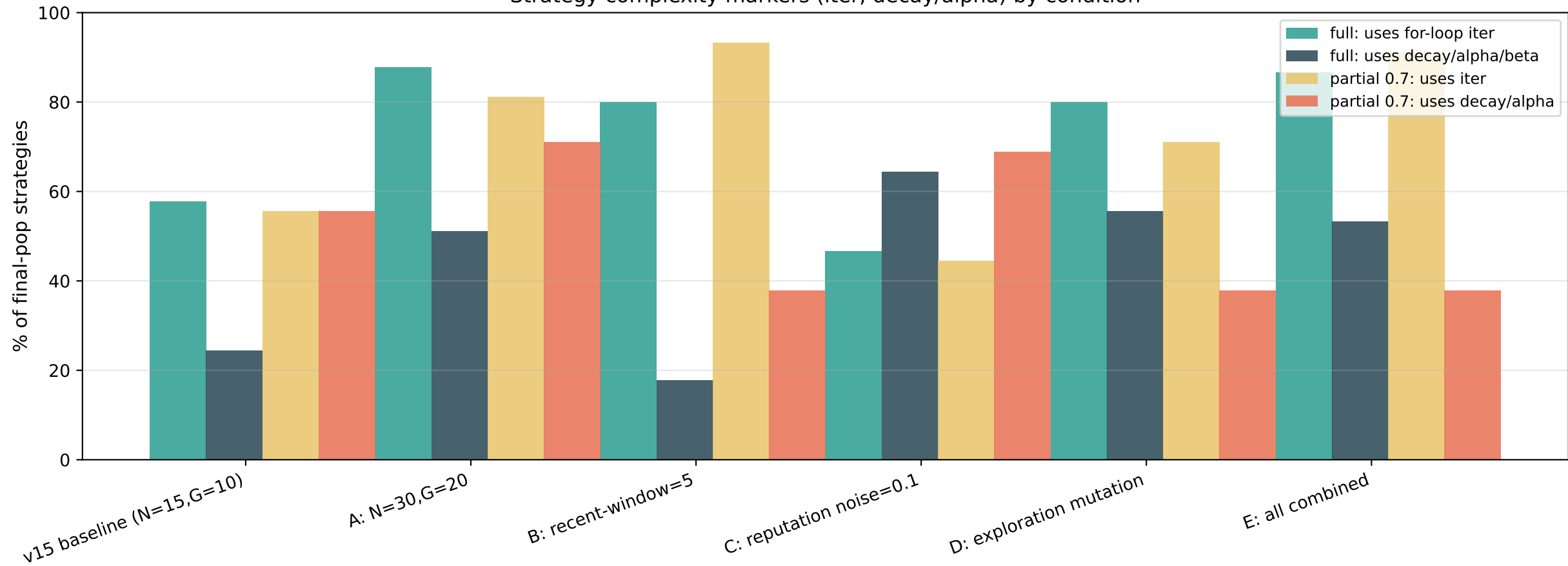
Strategy complexity markers (iter, decay/alpha) by condition
