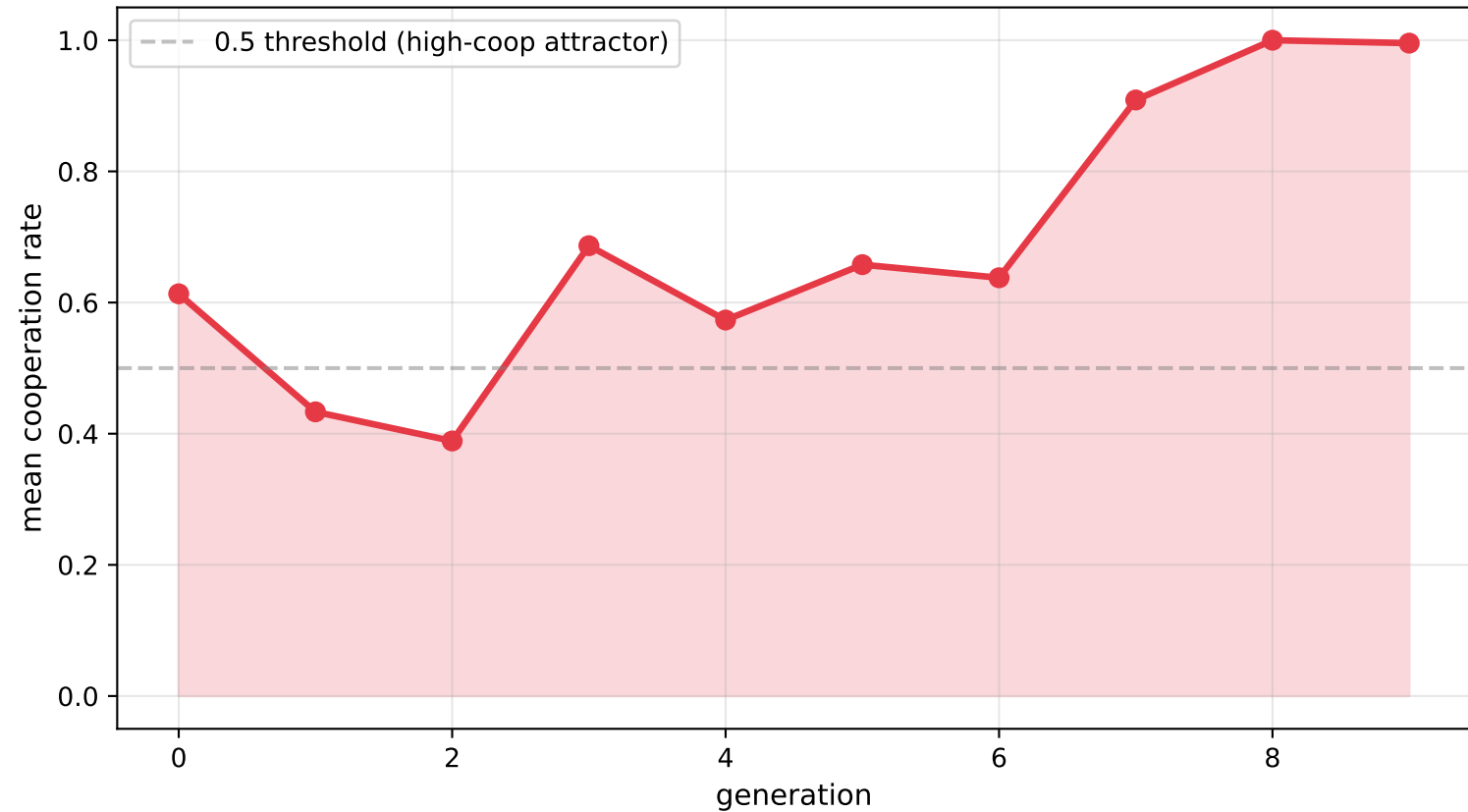
Highest-cooperation trajectory exp7/B_recent_window/partial_0.7_seed1 | final coop = 0.996
