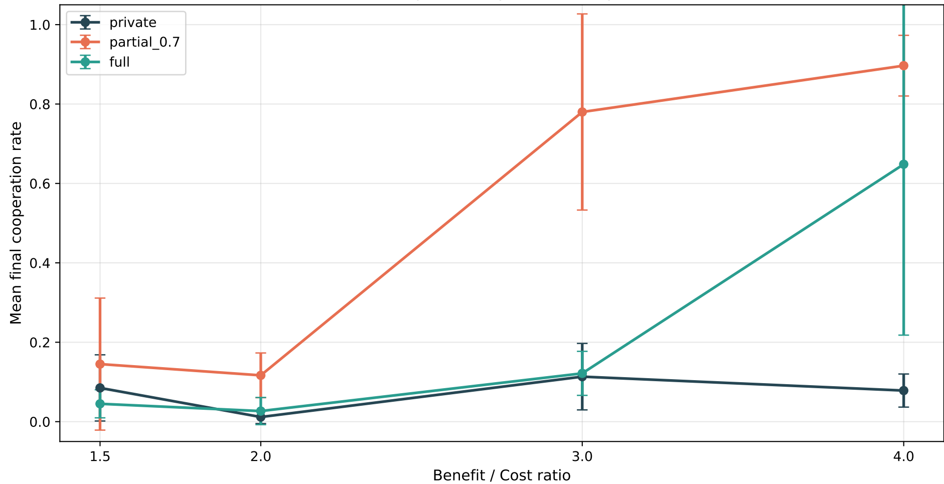
b/c ratio scan: cooperation by observability x benefit level
