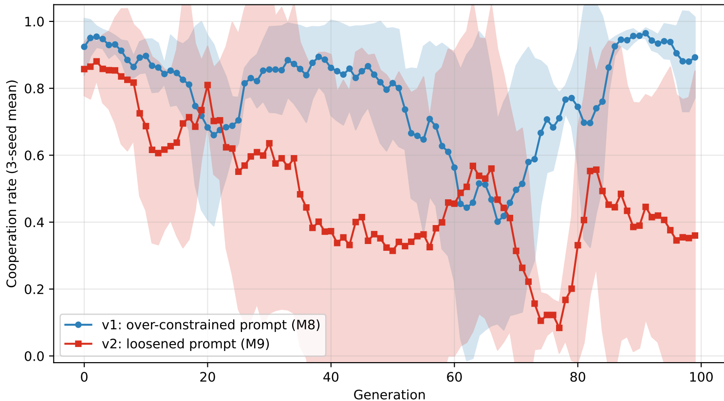
Fermi Z-like: prompt looseness reveals true evolutionary dynamics v1: mean 0.892 \pm 0.098 v2: mean 0.360 \pm 0.492 (M9)
