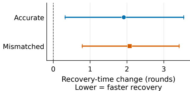
(a) Thinking OFF: Supplied CC Recovery
