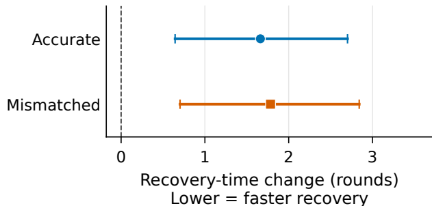
(c) Thinking OFF: Empty history Recovery
