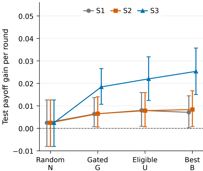
(a) Four fixed-pool policies Thinking OFF, post hoc
