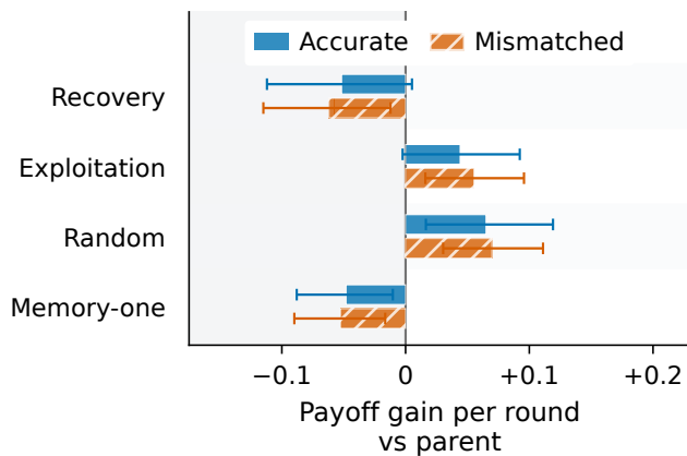
(a) Raw: Thinking OFF
