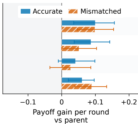
(b) Raw: Thinking ON
