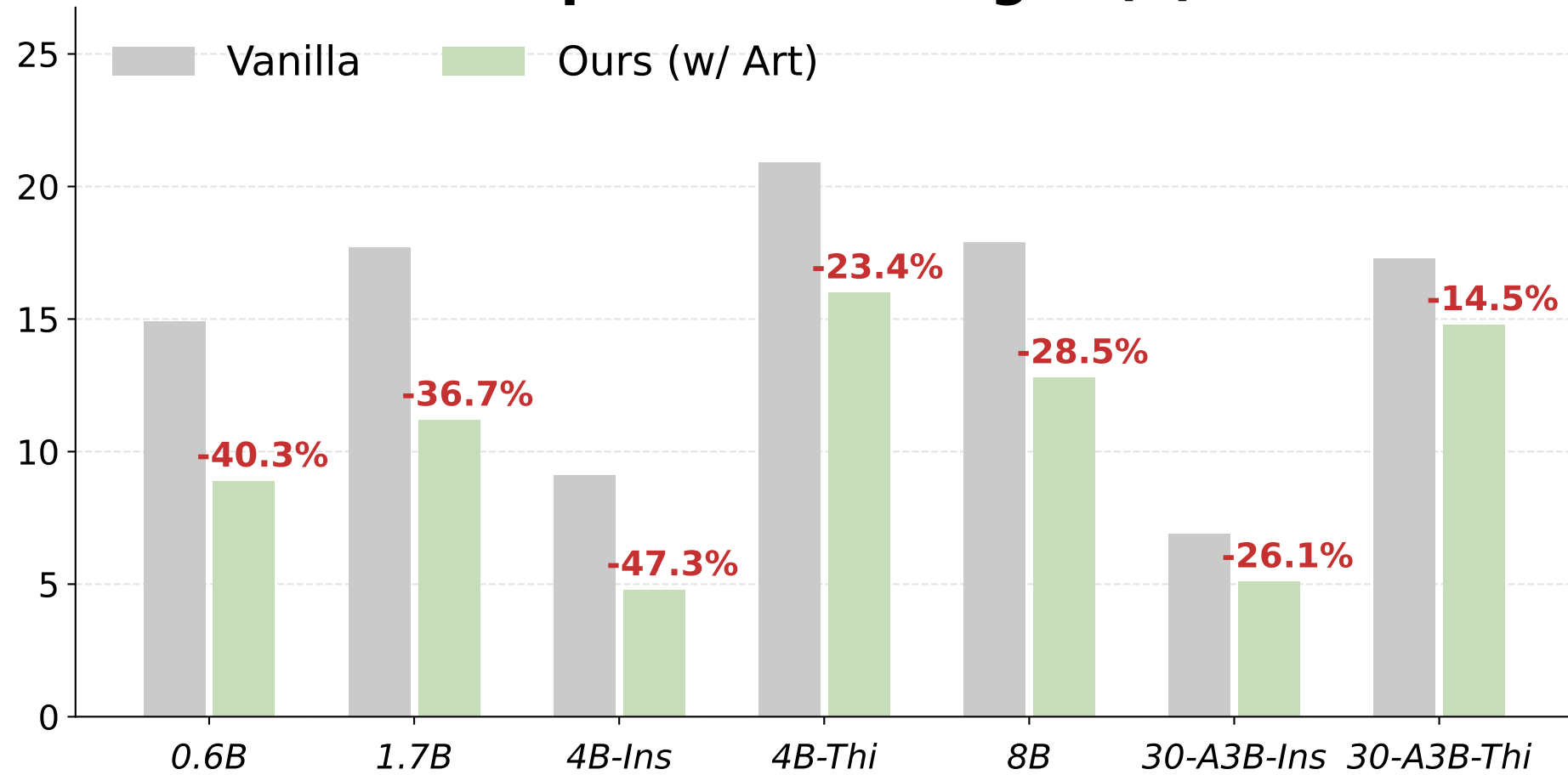
Output Token Length (k)
