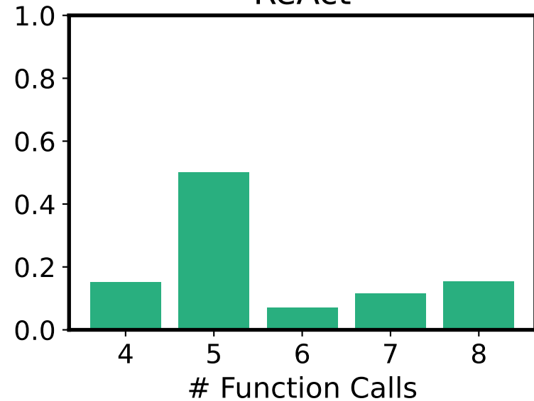
ReAct
