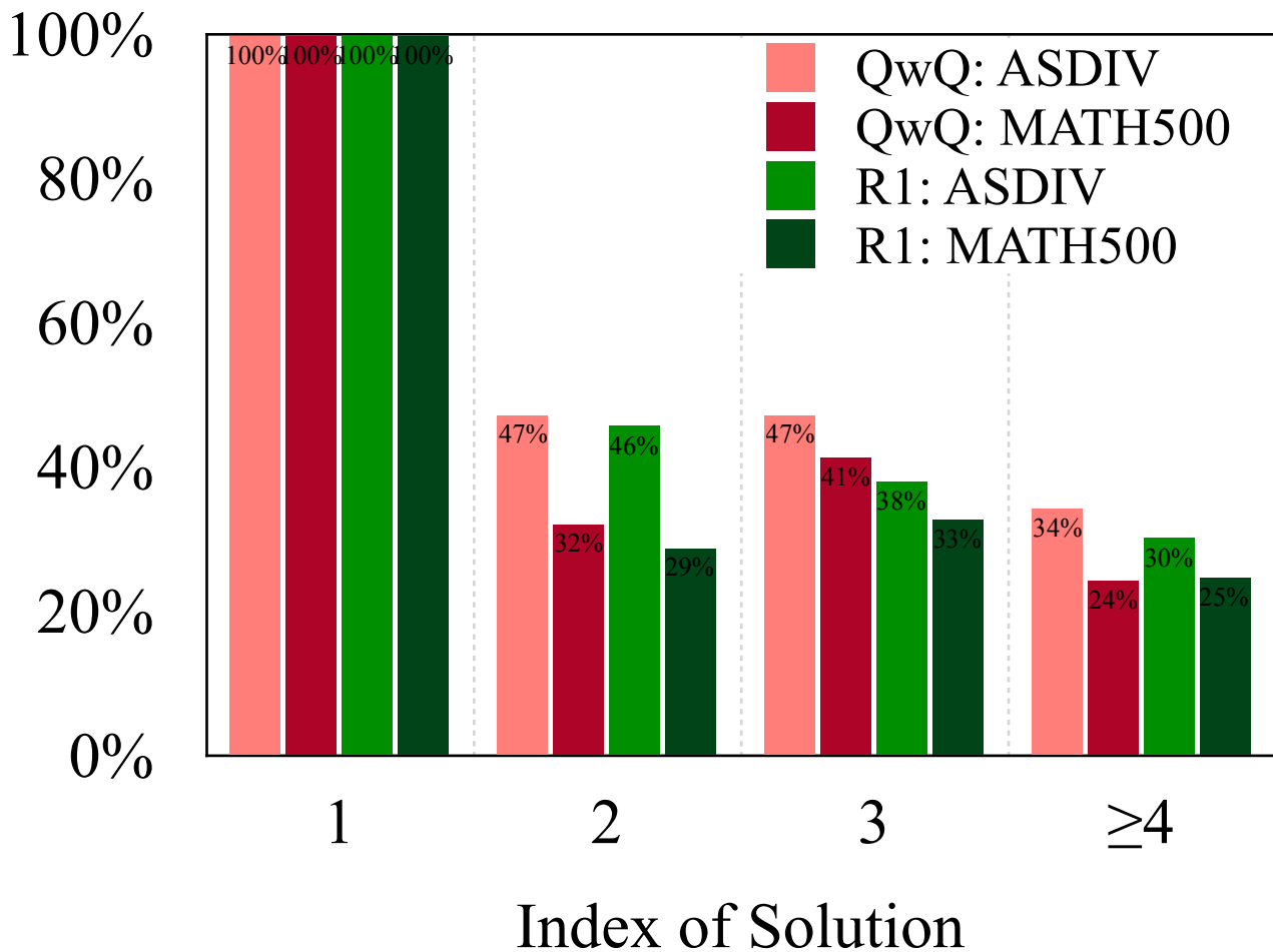
Distinctness Ratio
