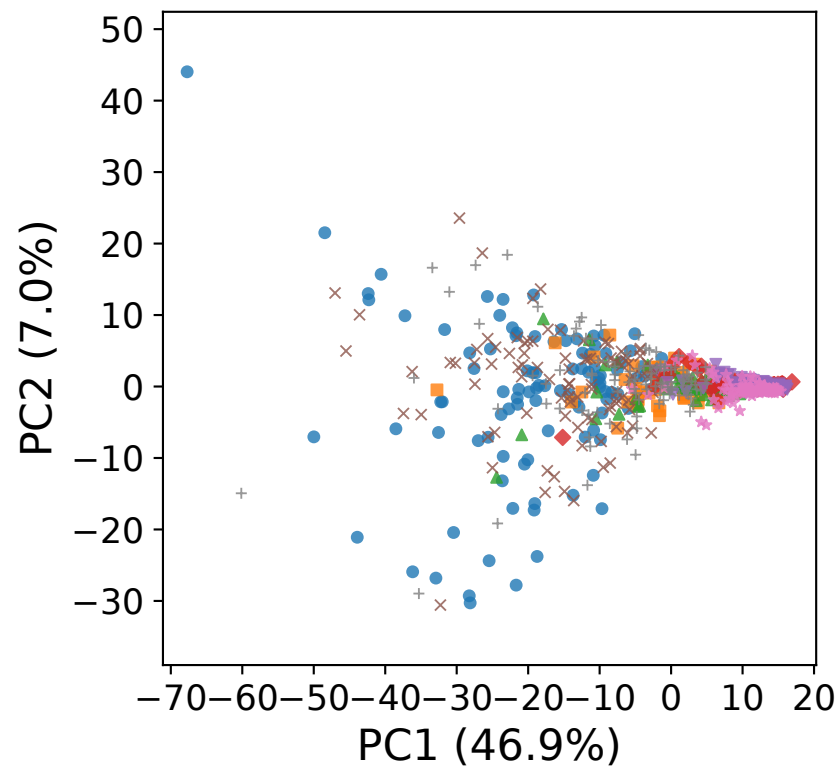
A STDP
