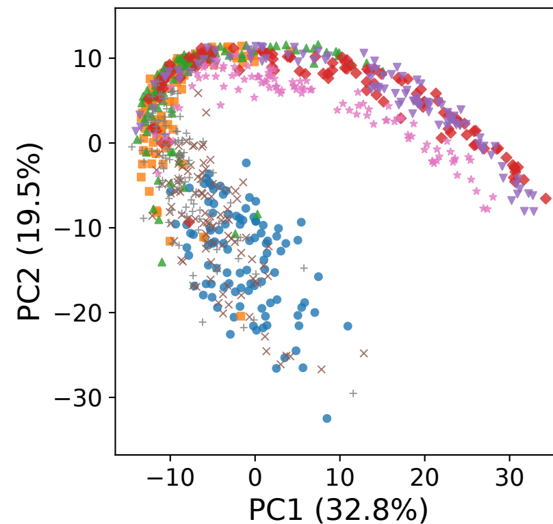
C SRDP
