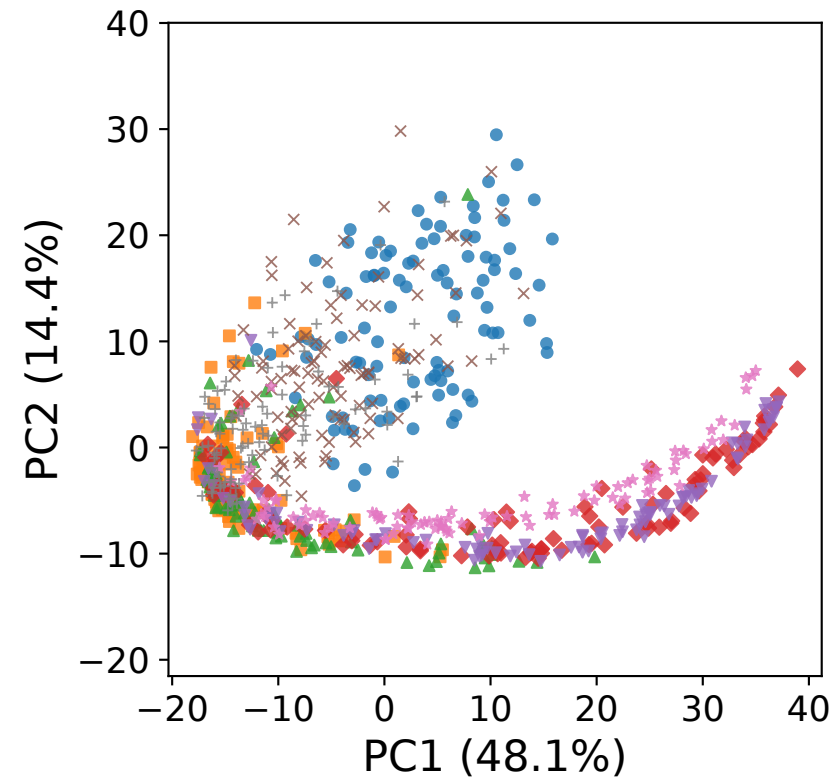
C SRDP
