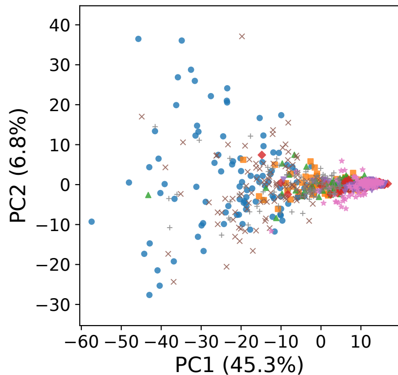
A STDP
