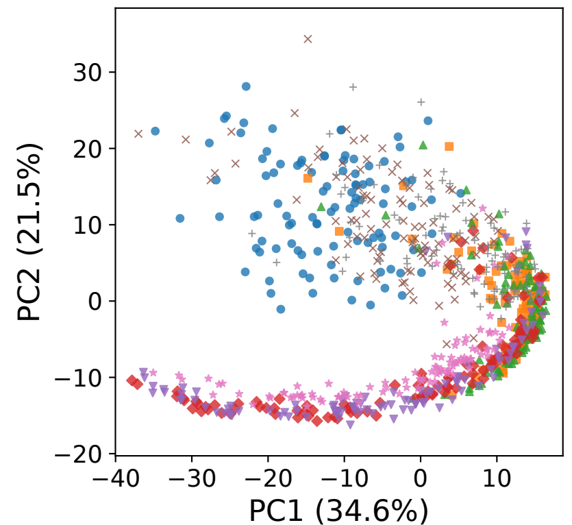
C SRDP
