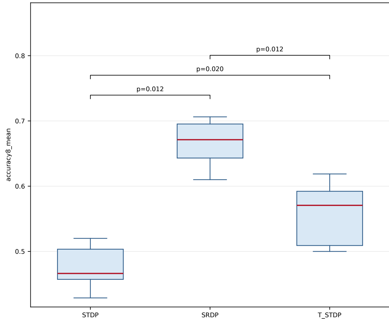
accuracy8_mean by learning rule with paired p-values
