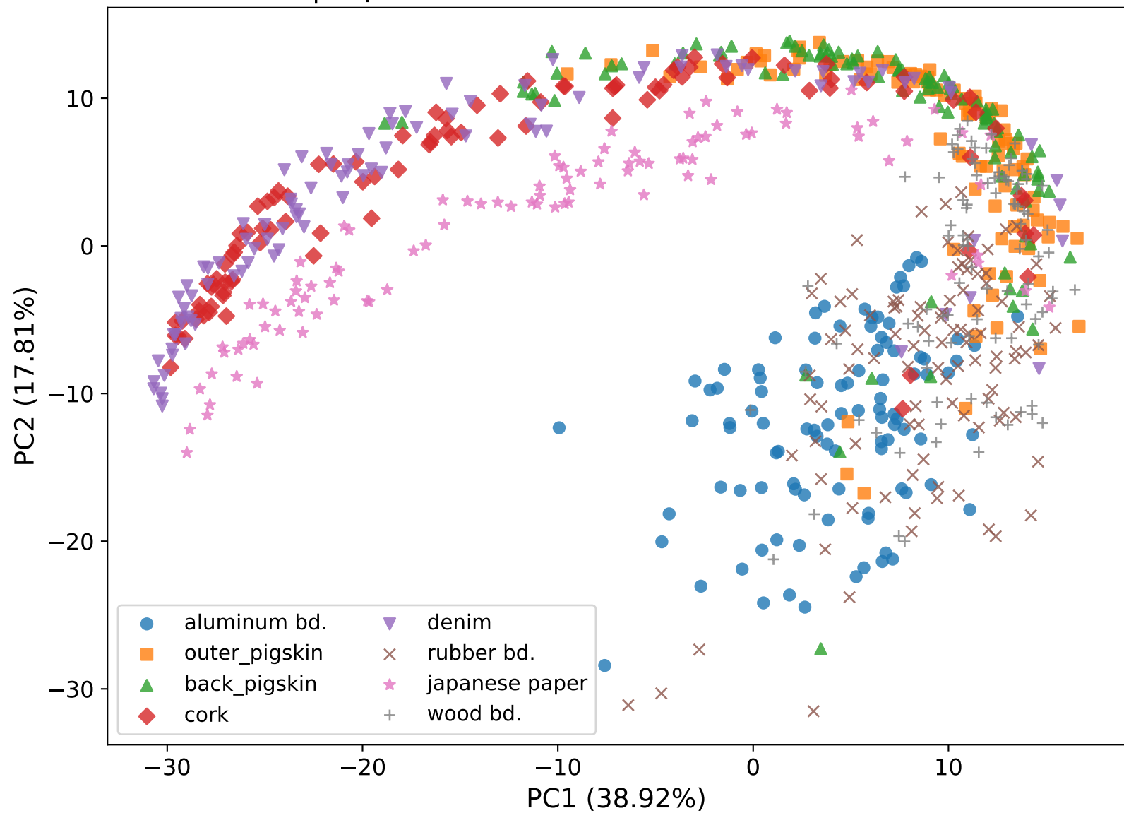
SRDP | explained variance: PC1=38.92%, PC2=17.81%
