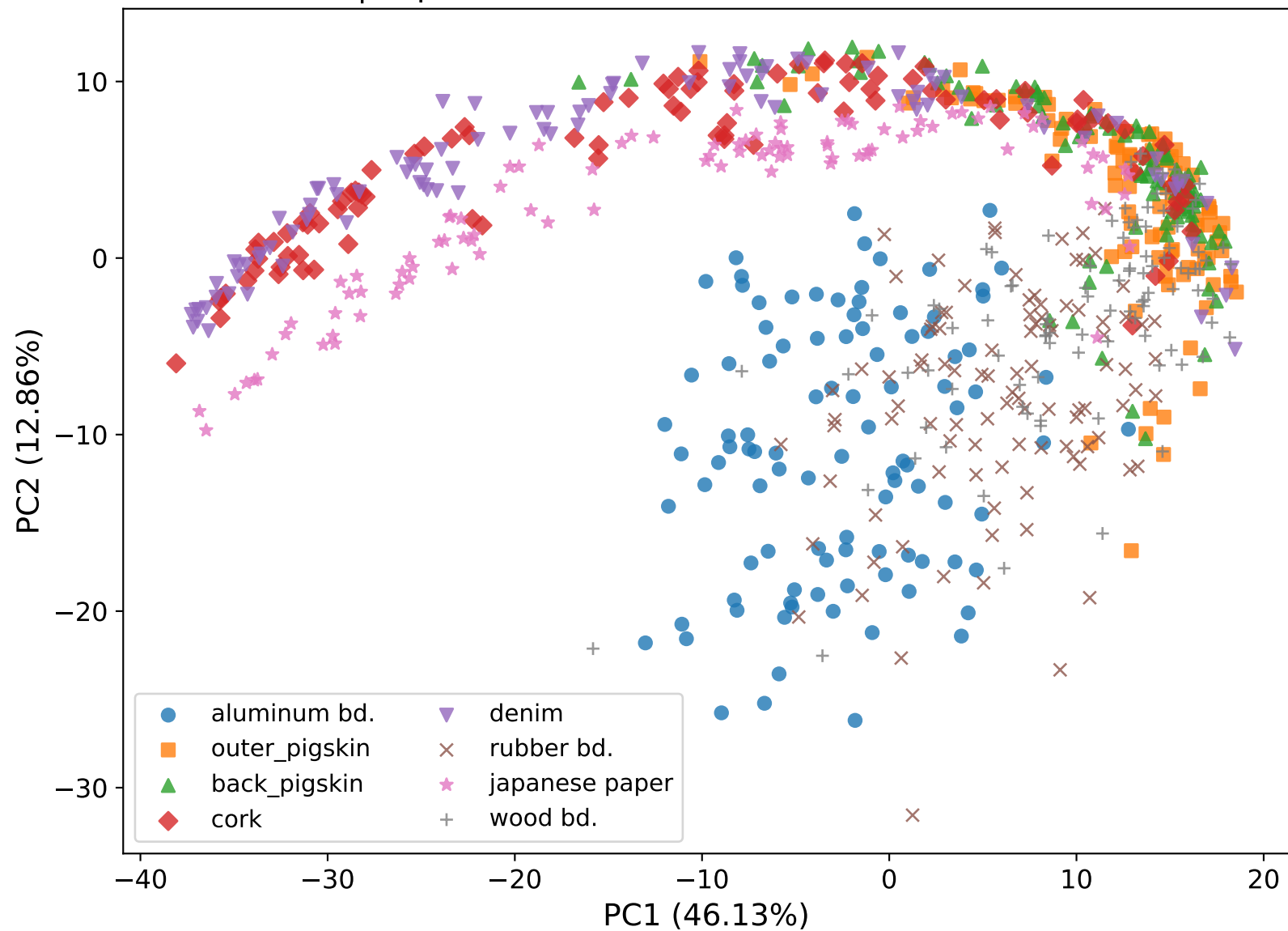
SRDP | explained variance: PC1=46.13%, PC2=12.86%
