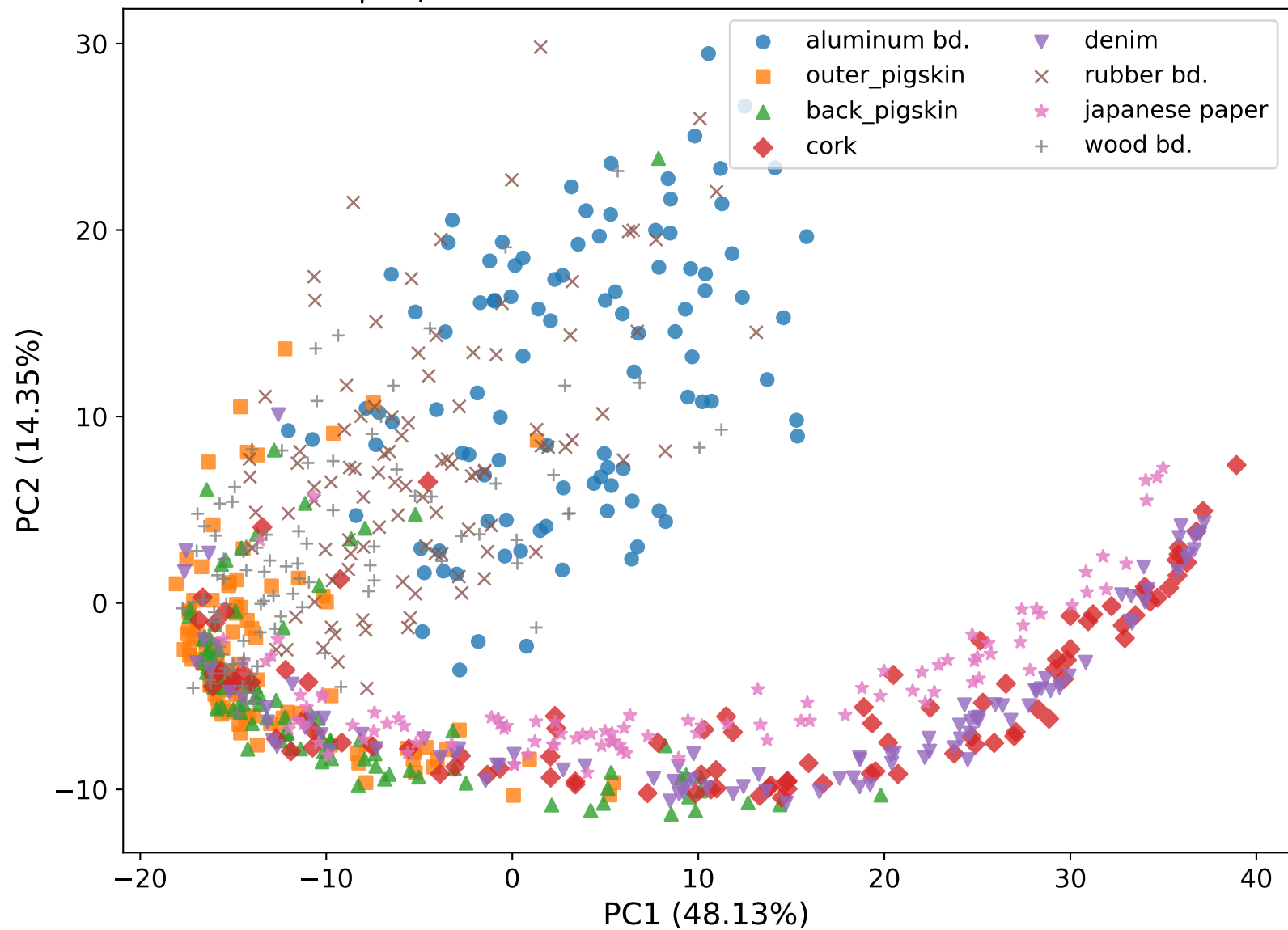
SRDP | explained variance: PC1=48.13%, PC2=14.35%
