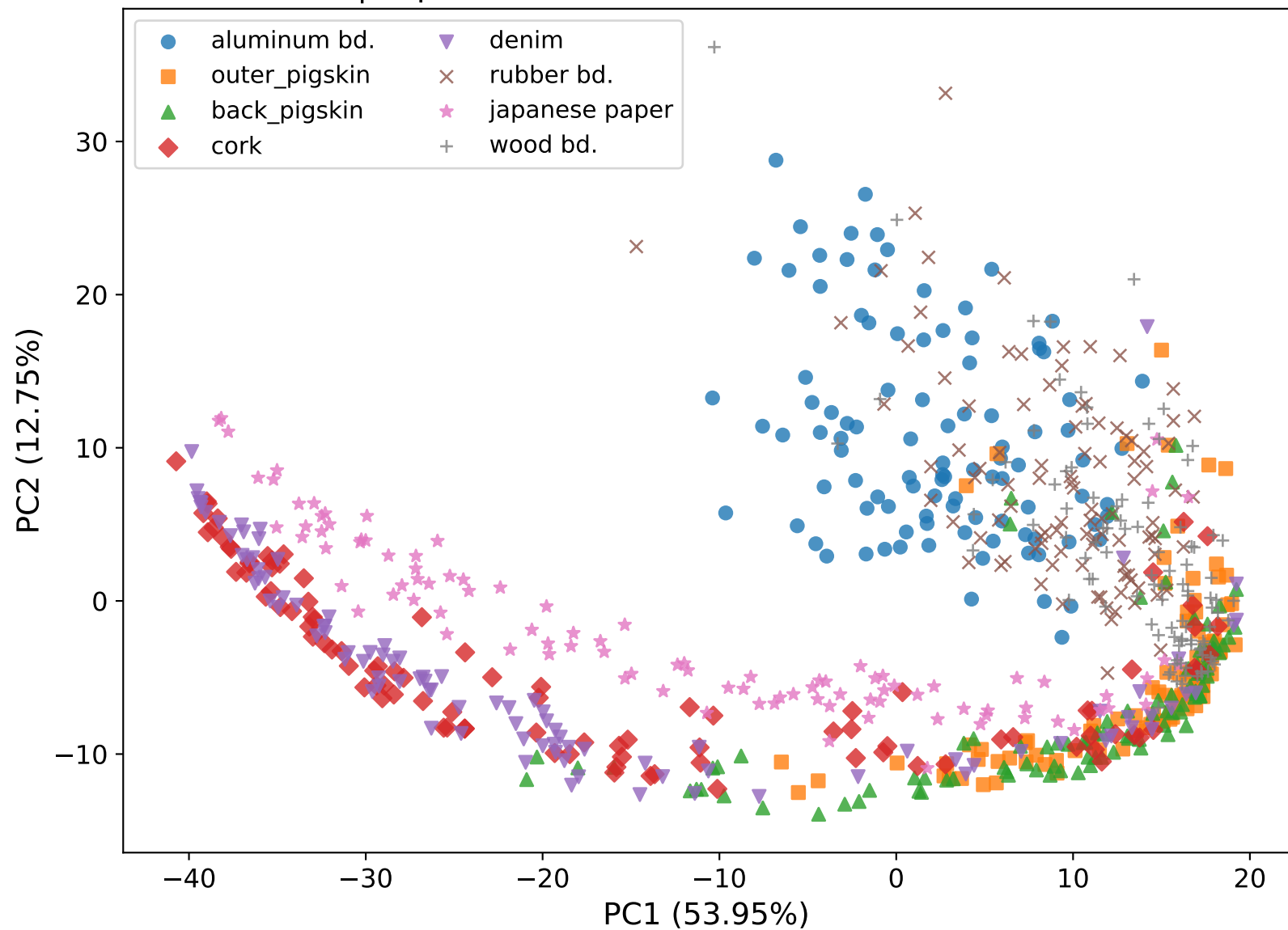
SRDP | explained variance: PC1=53.95%, PC2=12.75%
