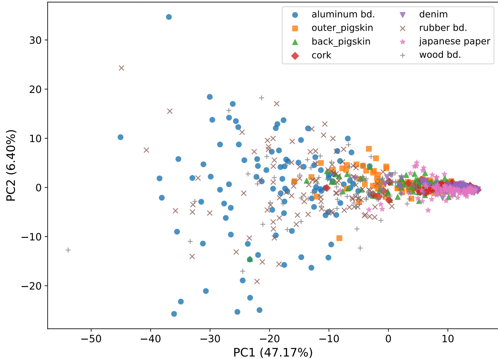
STDP | explained variance: PC1=47.17%, PC2=6.40%
