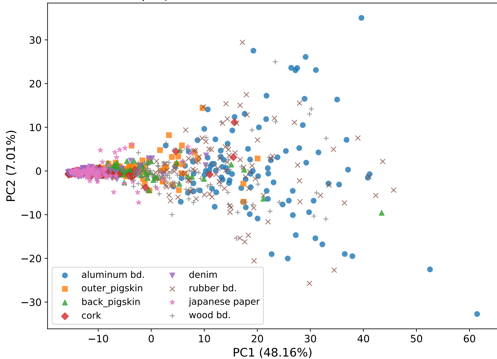
STDP | explained variance: PC1=48.16%, PC2=7.01%
