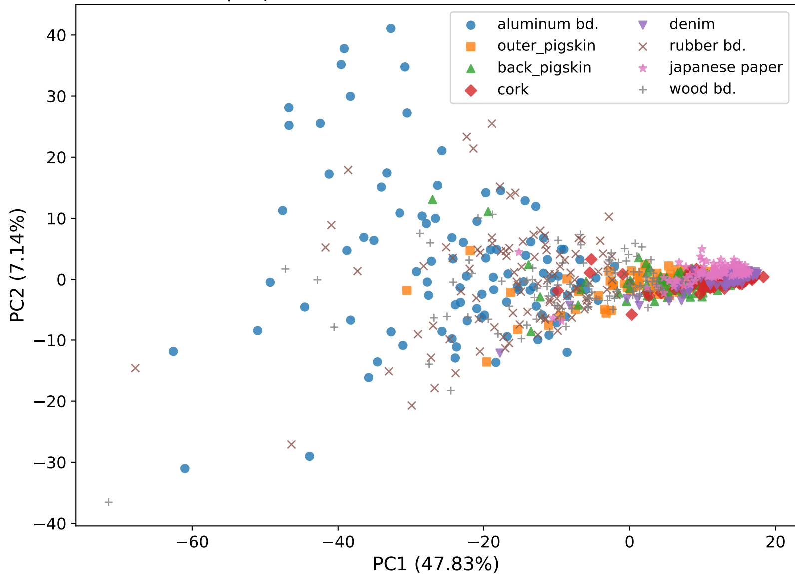
STDP | explained variance: PC1=47.83%, PC2=7.14%
