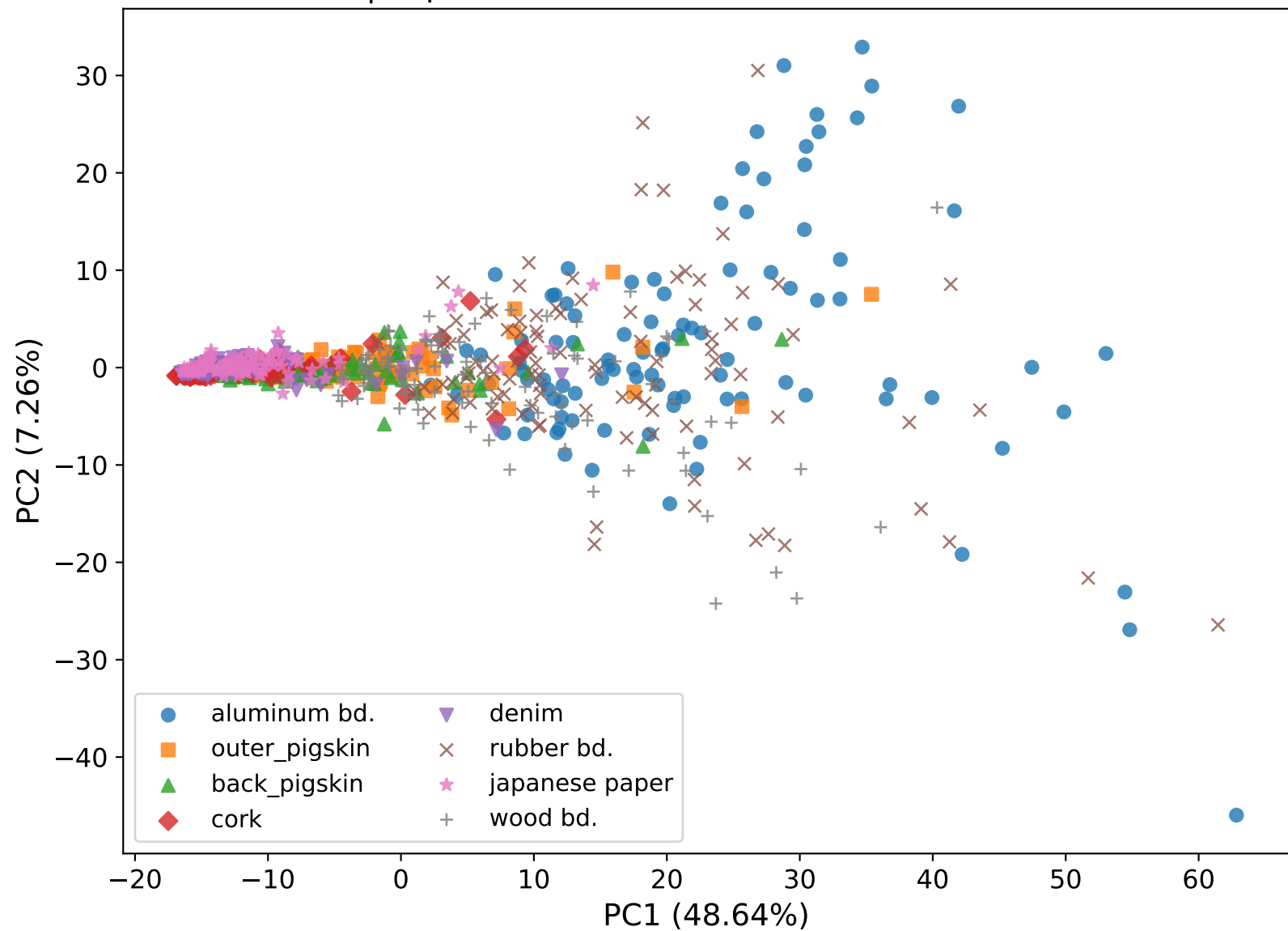
STDP | explained variance: PC1=48.64%, PC2=7.26%
