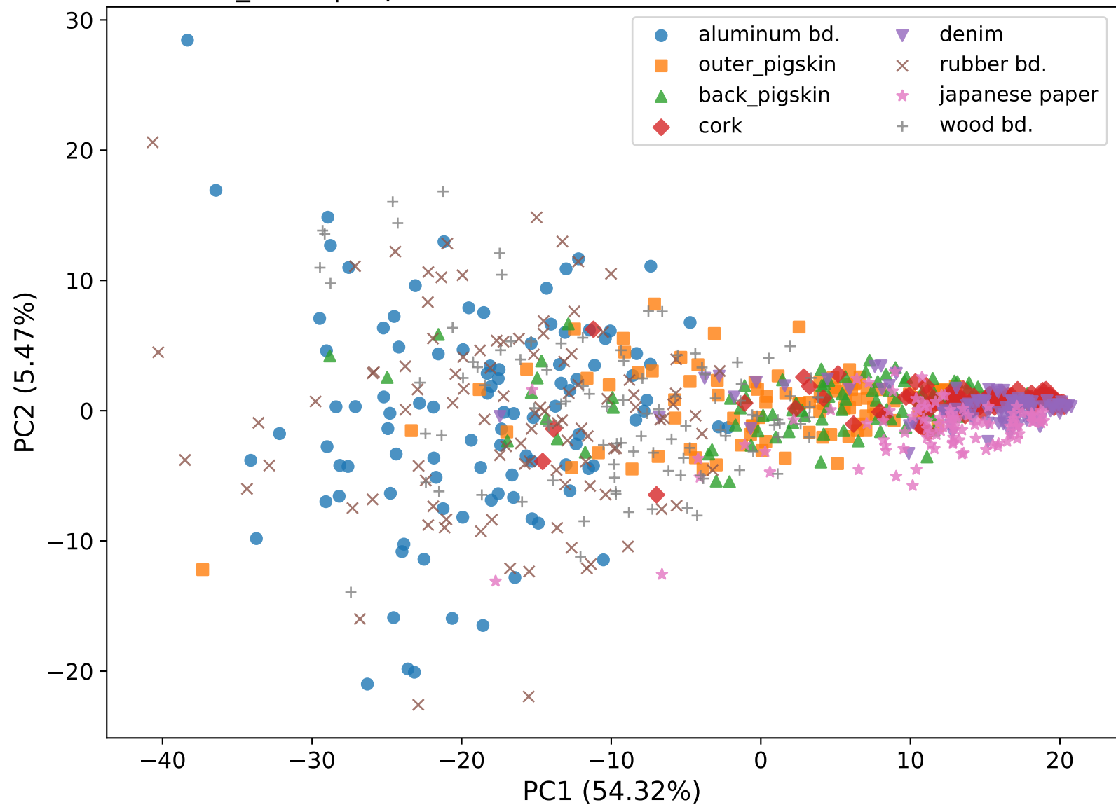
T_STDP | explained variance: PC1=54.32%, PC2=5.47%
