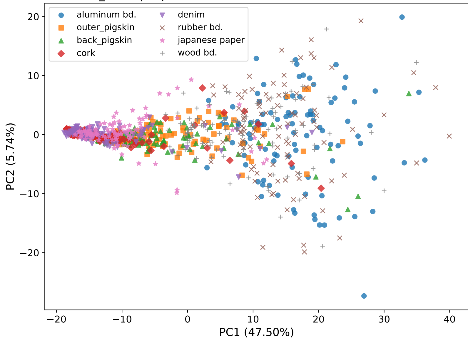
T_STDP | explained variance: PC1=47.50%, PC2=5.74%
