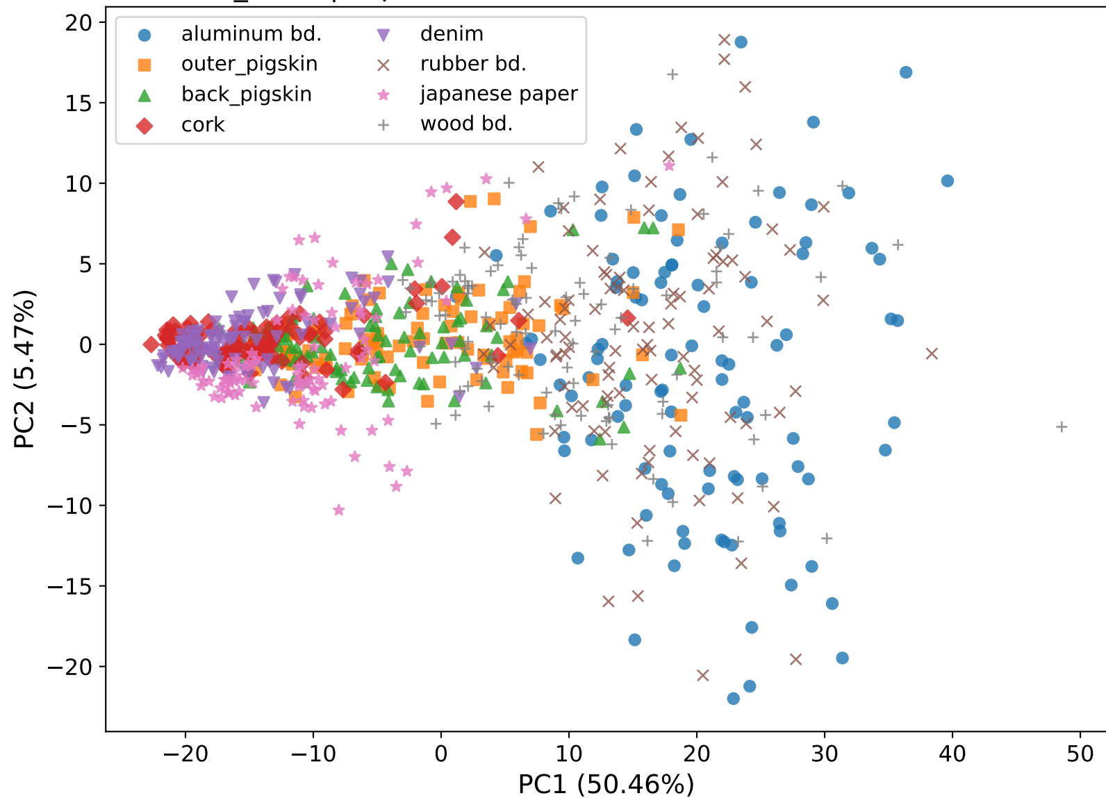
T_STDP | explained variance: PC1=50.46%, PC2=5.47%
