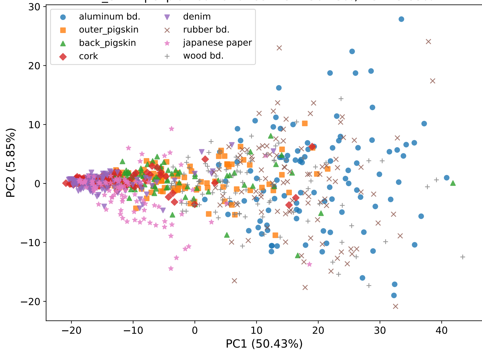
T_STDP | explained variance: PC1=50.43%, PC2=5.85%
