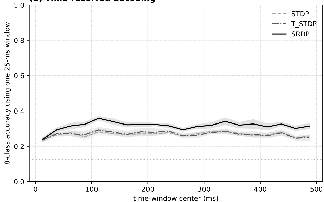
(b) Time-resolved decoding
