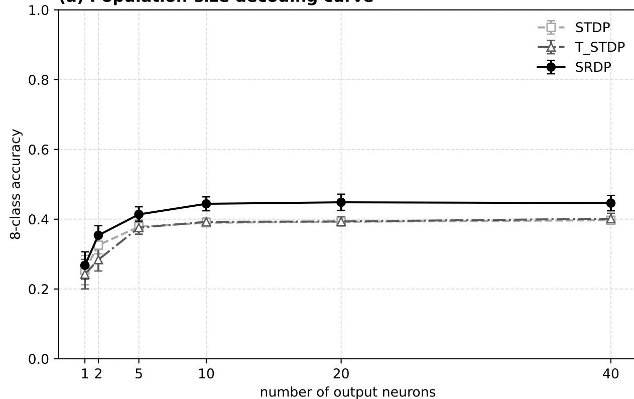
(a) Population-size decoding curve
