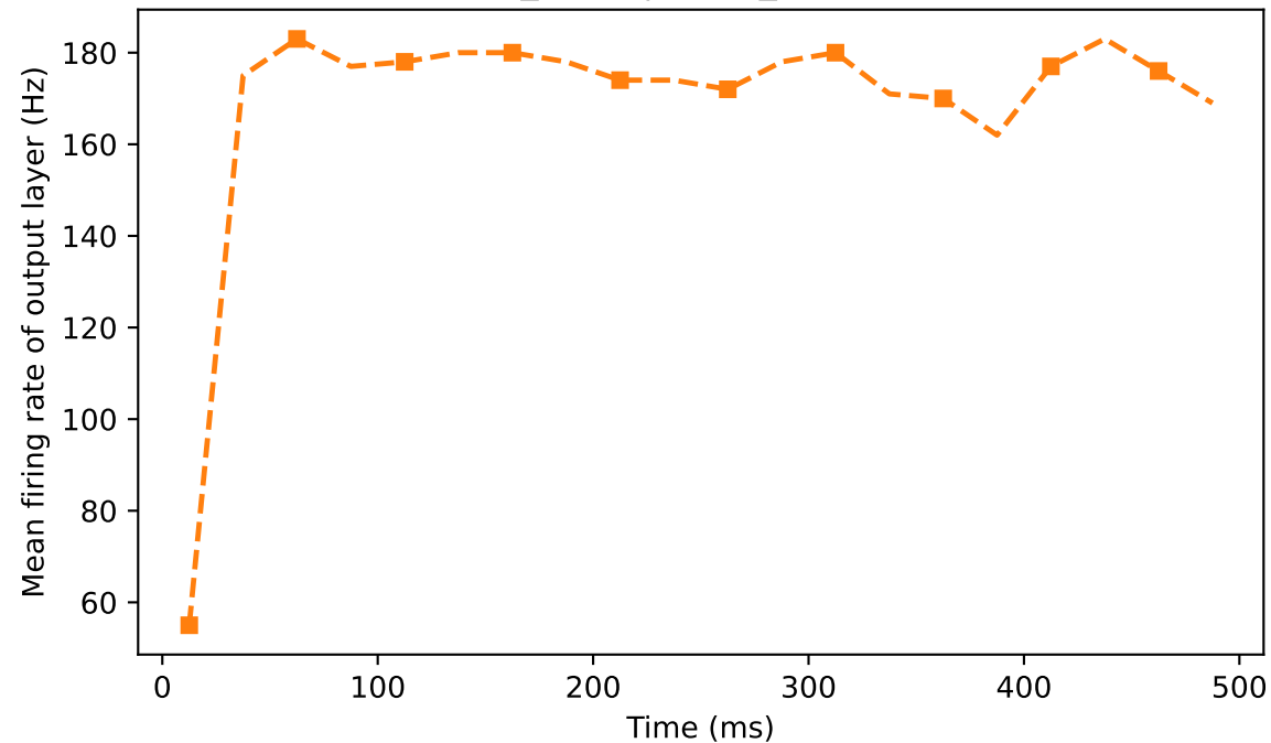
T_STDP | outer_pigskin
