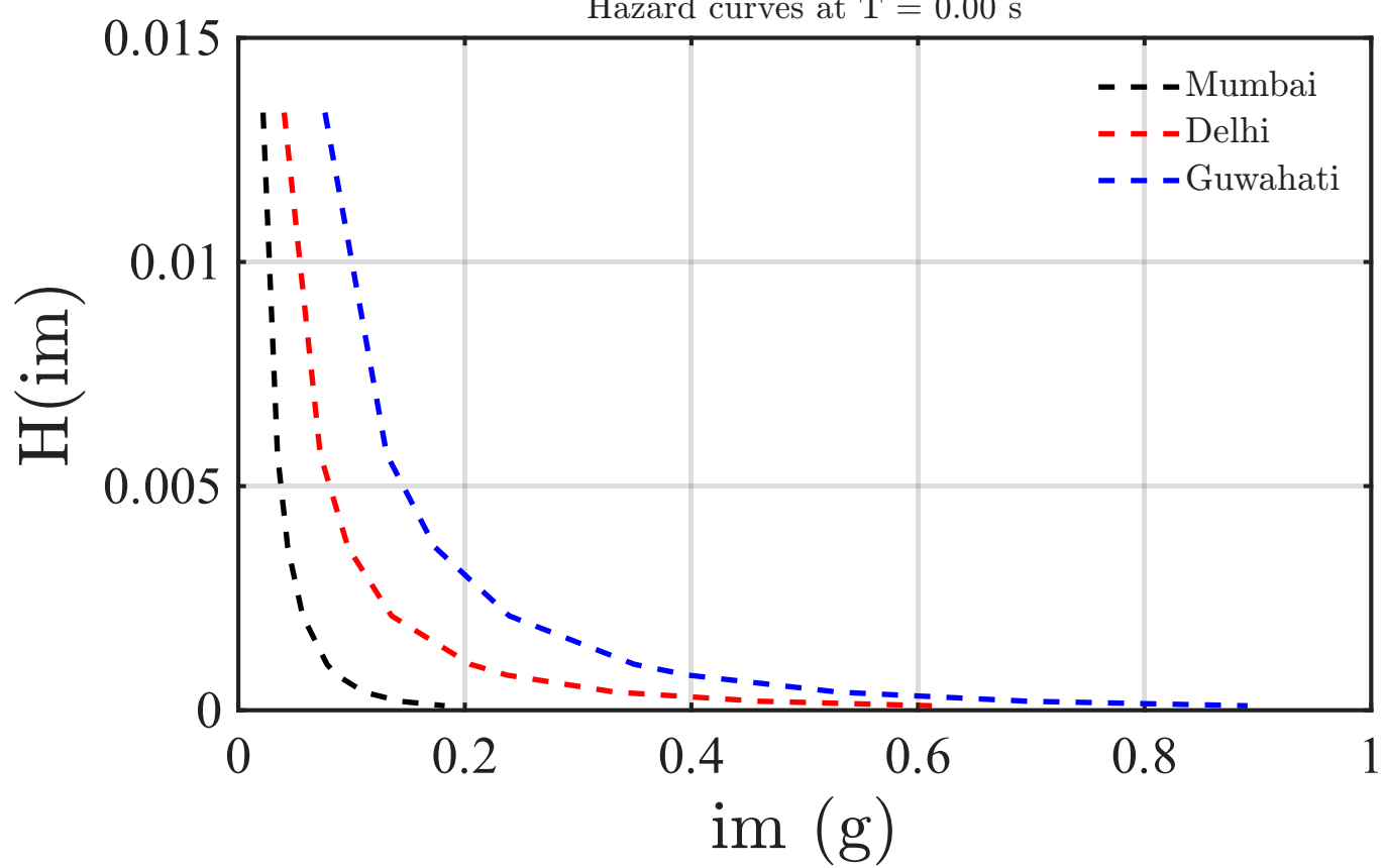
Hazard curves at T = 0.00 s
