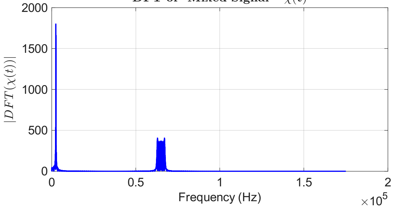
DFT of Mixed Signal – \chi(t)
