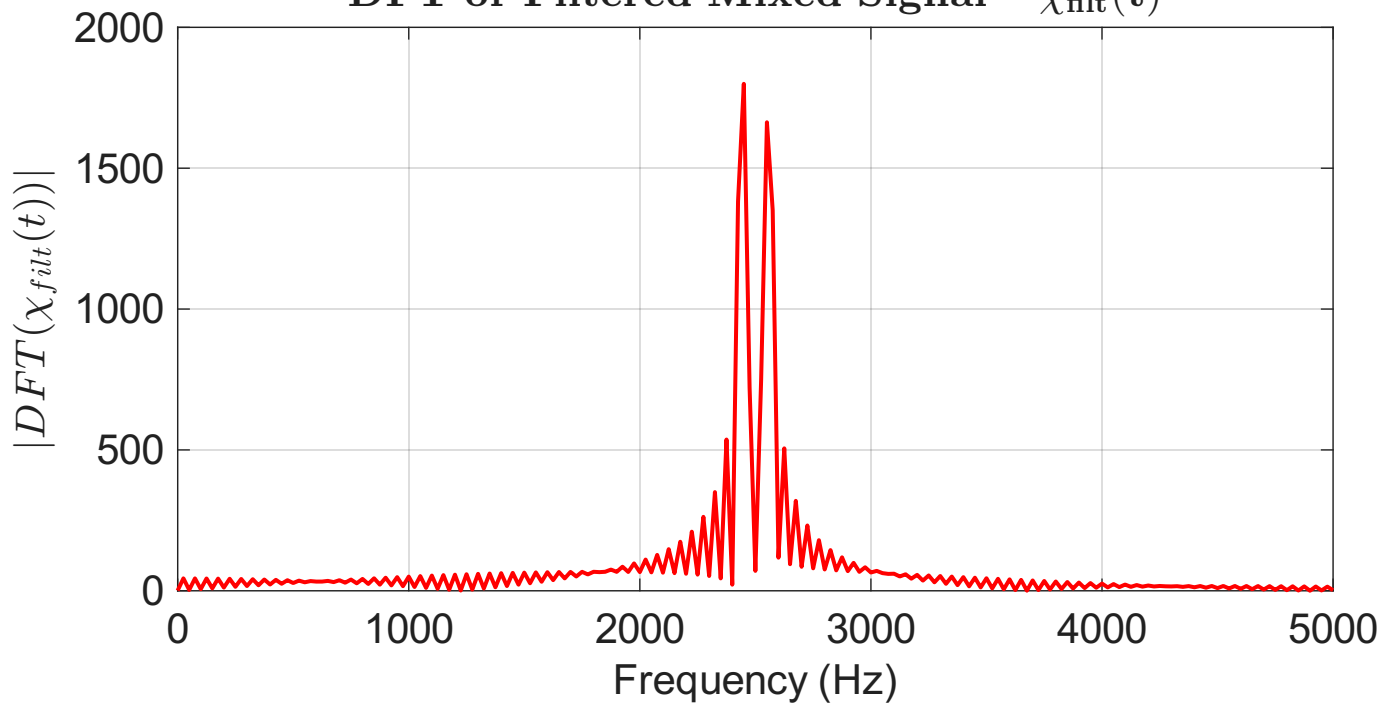
DFT of Filtered Mixed Signal – \chi_{\text{filt}}(t)
