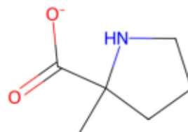
Rank 16 anion
