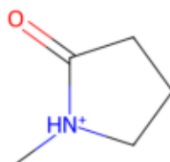
Rank 20 cation
