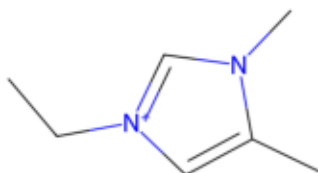
Rank 15 cation
