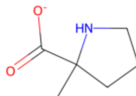
Rank 8 anion
