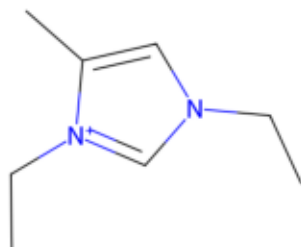
Rank 12 cation
