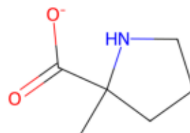
Rank 12 anion
