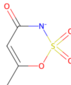
Rank 20 anion
