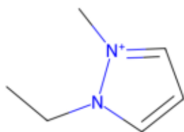
Rank 8 cation
