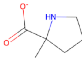
Rank 15 anion
