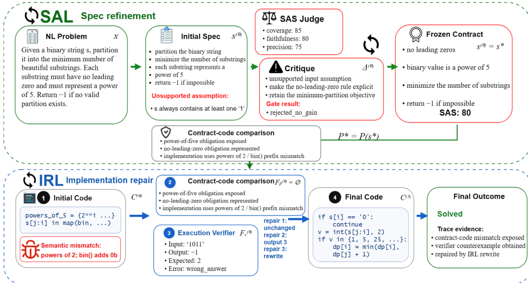
Figure 3: Case-study trace for problem 2883.
