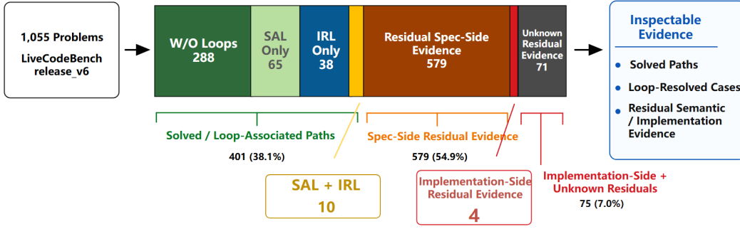
Figure 2: Final-aligned trace evidence.
