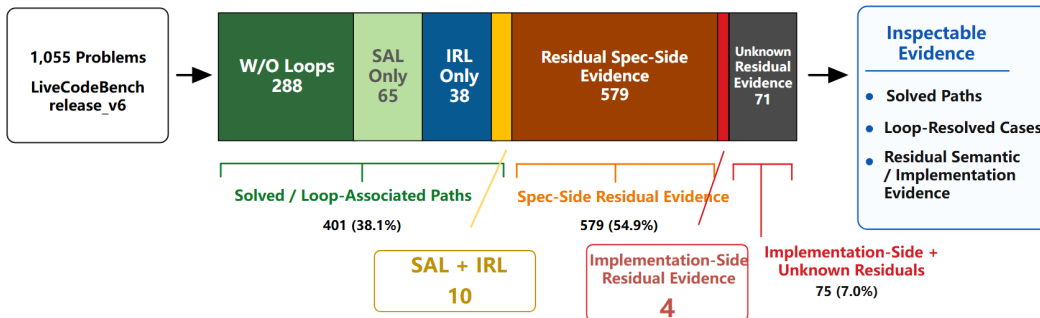
Figure 2: Final-aligned trace evidence on 1,055 LiveCodeBench release_v6 problems.
